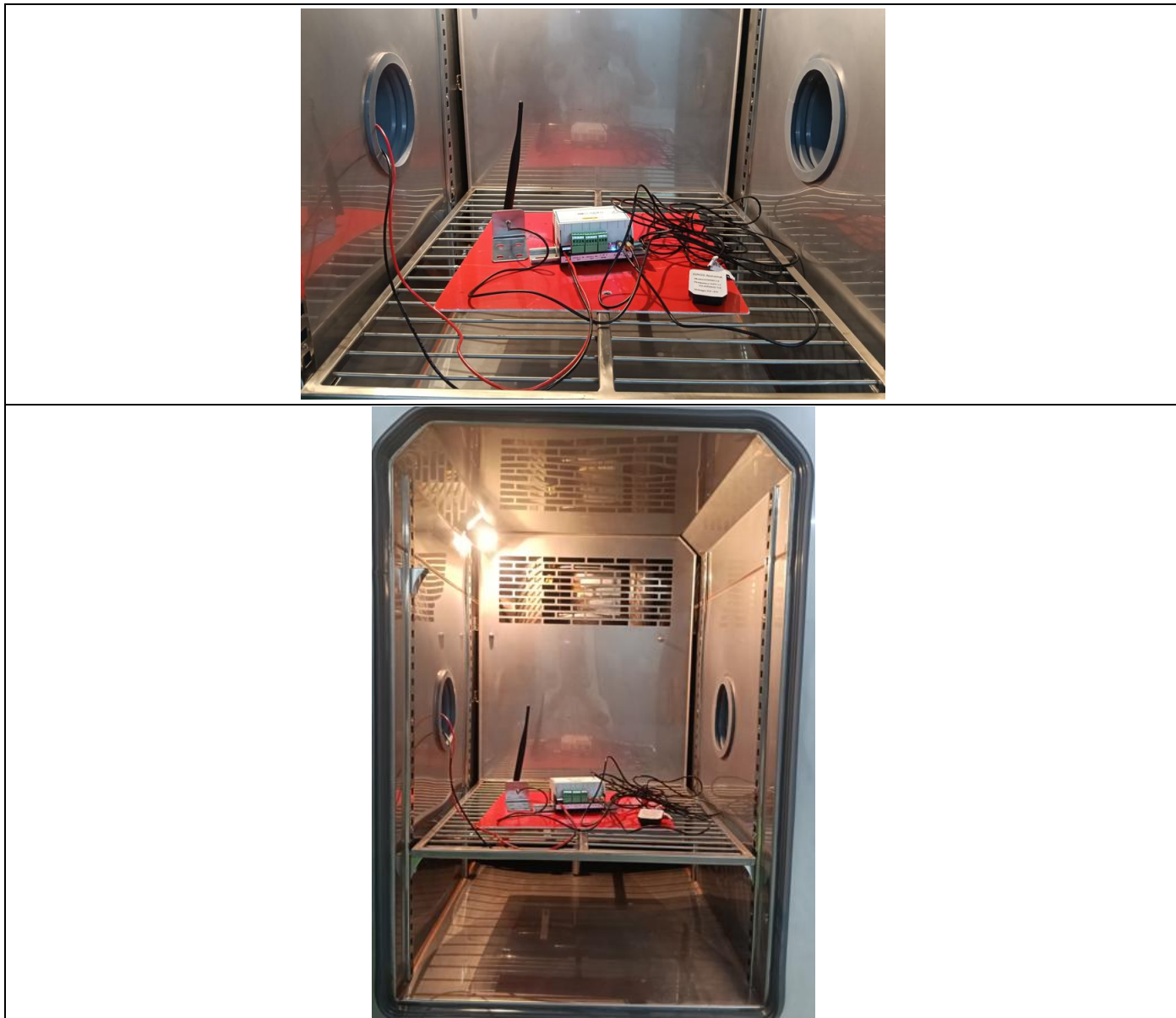
Figure 2: Dry Heat Test Setup Photo
