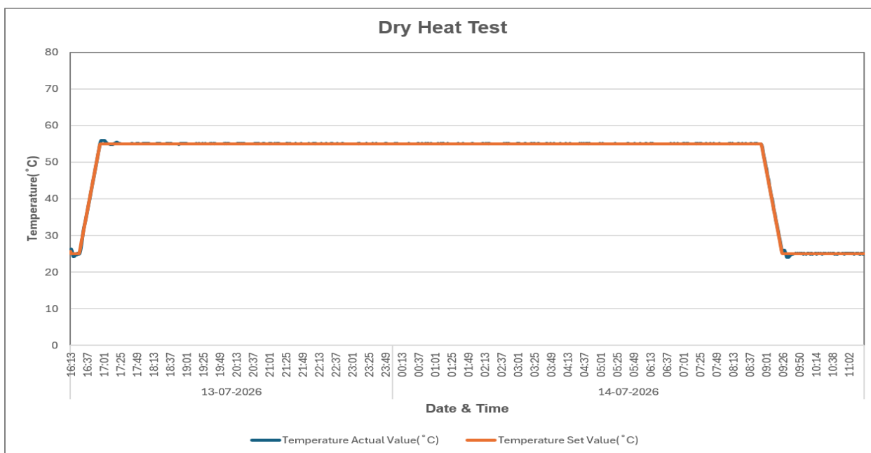
Figure 3: Dry Heat Test Graph
