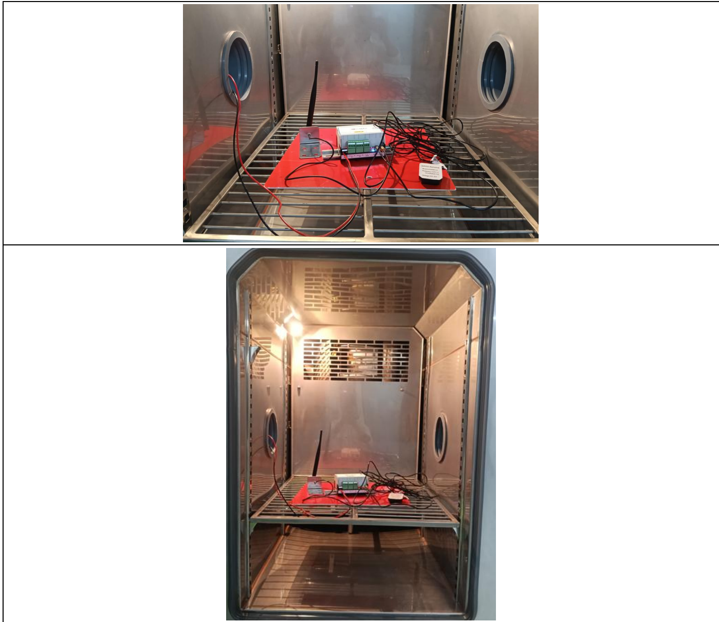
Figure 2: Damp Heat Steady State Test Setup Photo
