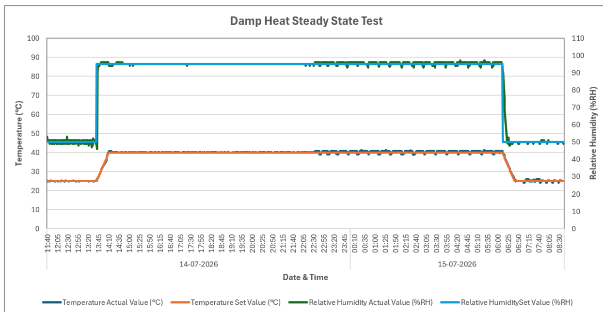
Figure 3: Damp Heat Steady State Test Graph
