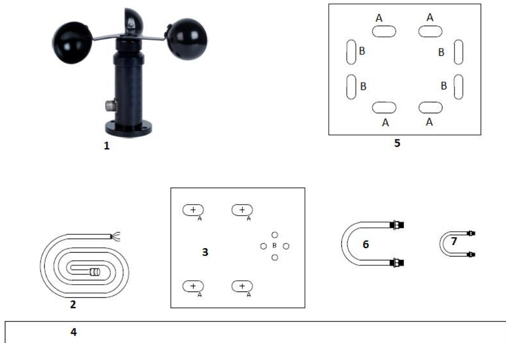
Fig: 1.1 – Wind Speed Sensor along with mounting
