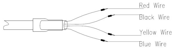
Fig: 4.1 – Wind Speed Sensor Wire
