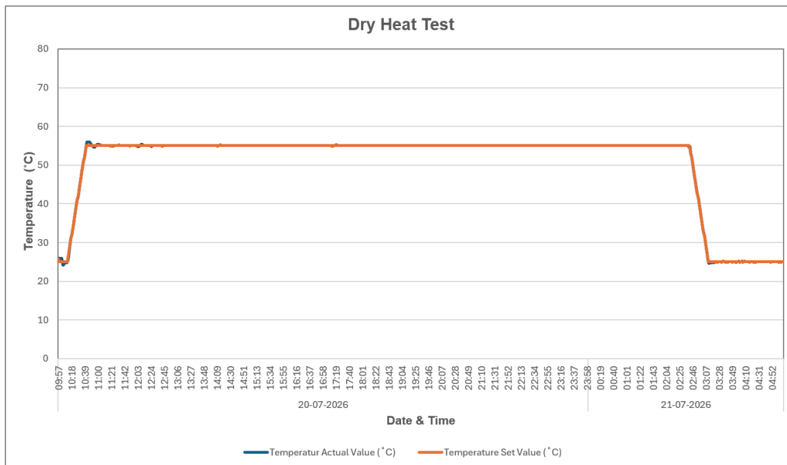
Figure 3: Dry Heat Test Graph
