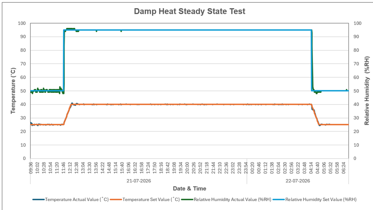
Figure 3: Damp Heat Steady State Test Graph
