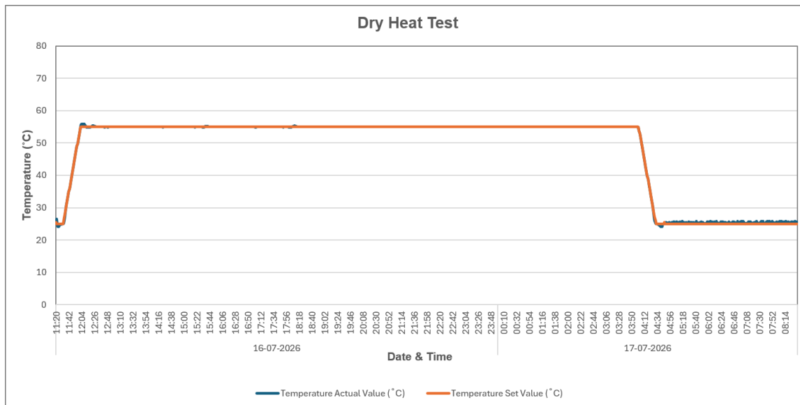
Figure 3: Dry Heat Test Graph
