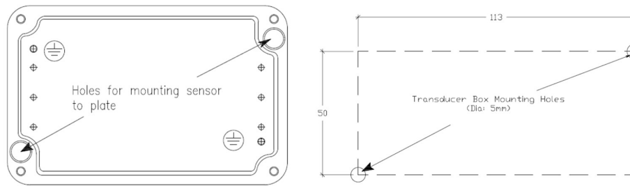
Fig – 4.3: Holes for fixing sensor to mounting plate.
