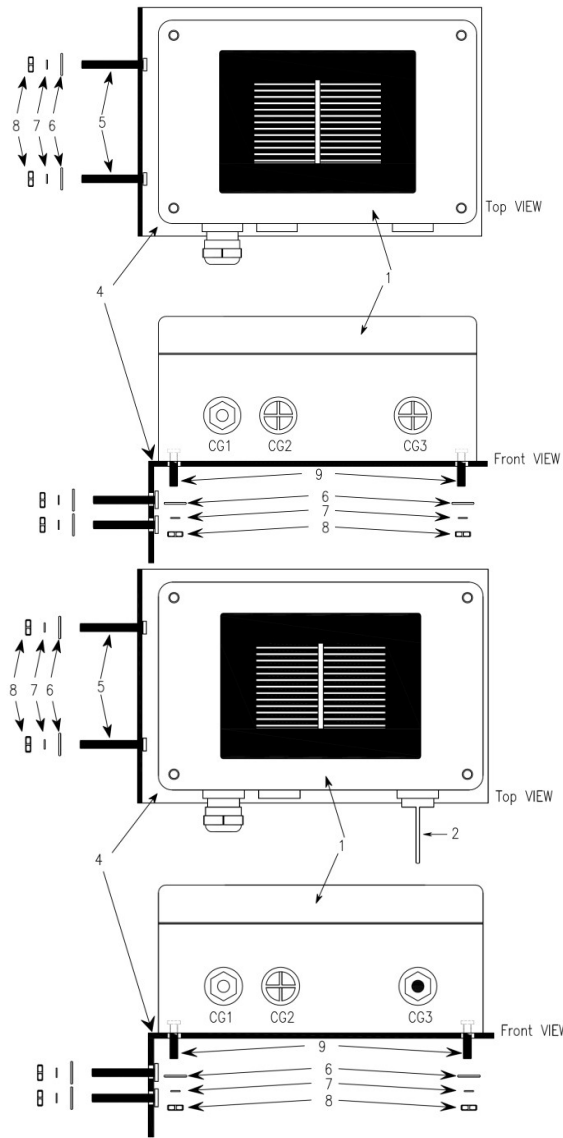
Fig-3.1: MBMet-500AB Parts
