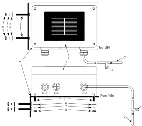
Fig-3.3: MBMet-500CB Parts
