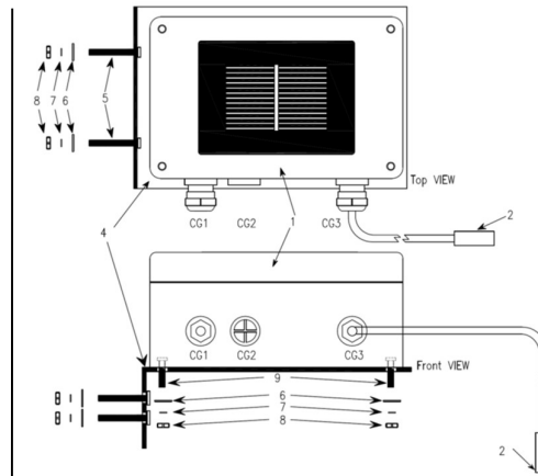
Fig-3.4: MBMet-500DB Parts
