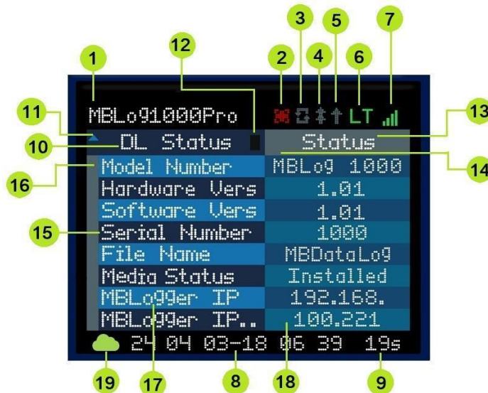
Figure-4.3: Datalogger OLED
