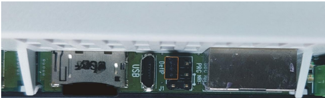
Figure -5.1: Jumpers for setting default IP address in the datalogger HW version 3.1.
