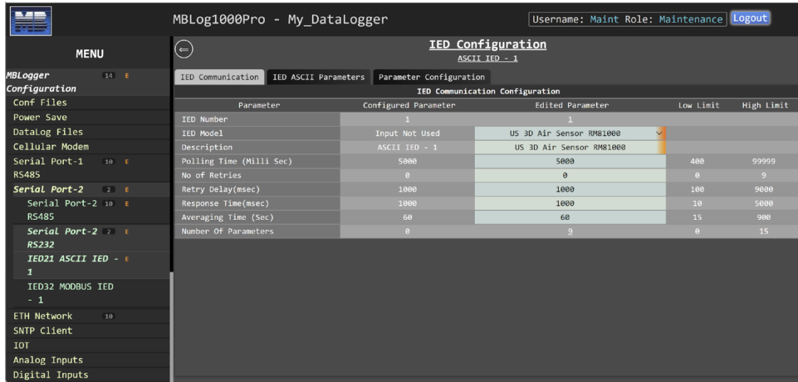
Figure-6.13.1: Configuration of ASCII IED communication parameters.
