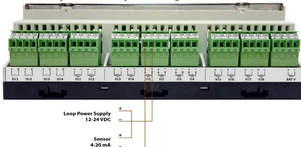
Figure-3.10: Measurement mA (4-20mA) input connections.
