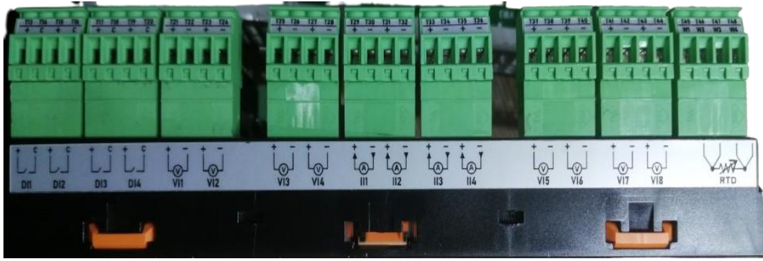
Figure-3.1.5: MBLLogger signal input terminals (For Hardware version 5.11)
