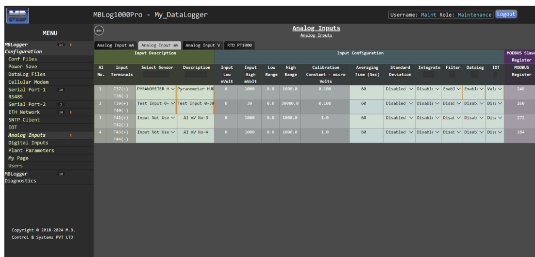
Figure-6.16.2: Configuration of mV input channels.
