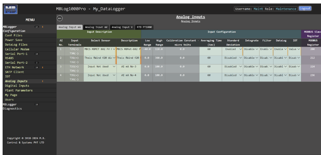
Figure-6.16.1: Configuration of mA input channels.
