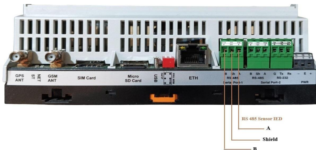
Figure-3.3: MBLLogger serial port-1 (RS485) connections.
