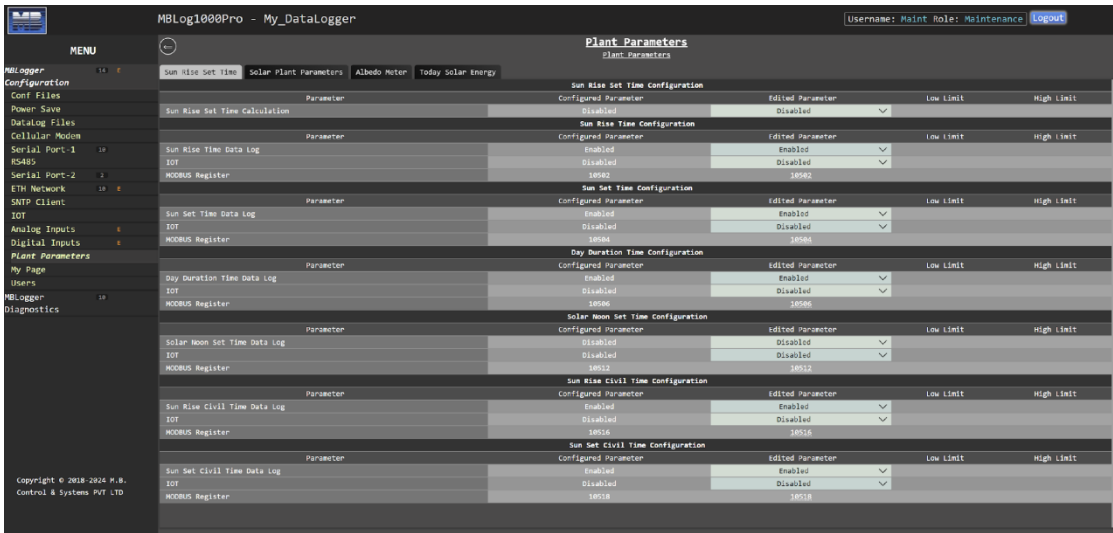
Figure-6.21.1: Configure Sun Rise and Set Time parameters.
