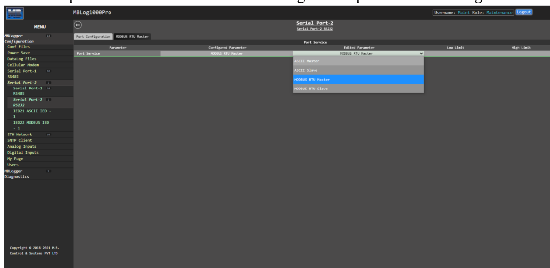
Figure-6.10.2: Configuration of serial port-2 RS232.
