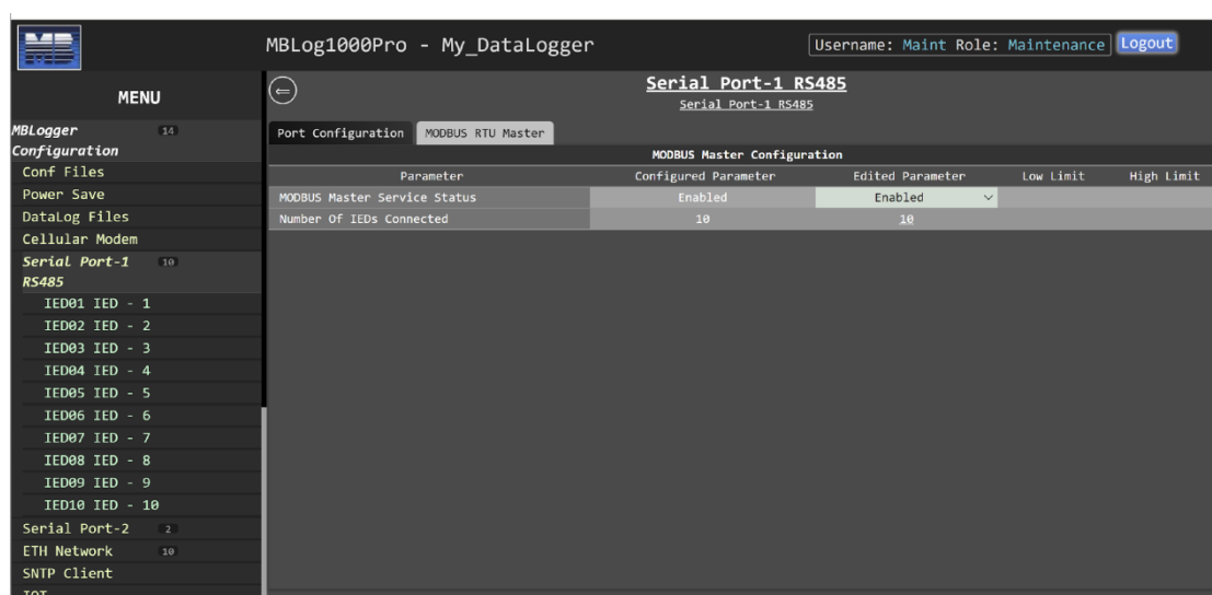
Figure-6.9: Configuration of serial port-1 RS485.
