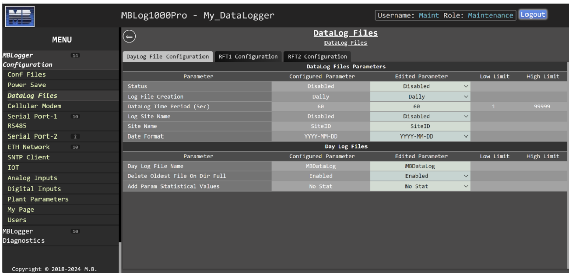
Figure-6.5.1: Log file Configuration
