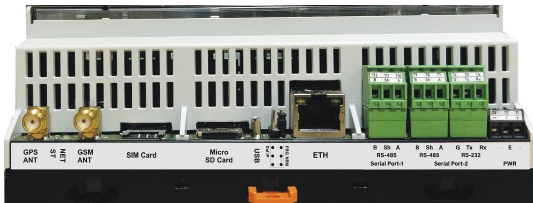
Figure-3.1.3: MBLLogger communication port and terminals (For Hardware version 3.11)
