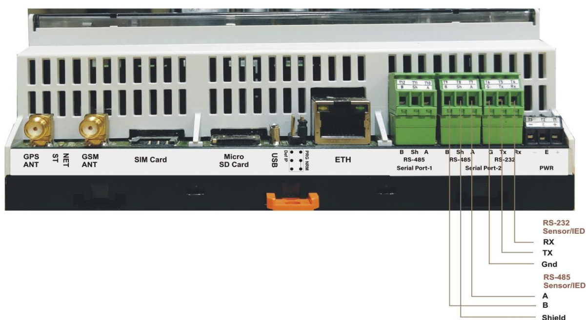
Figure-3.4: MBLLogger serial port-2 (RS485 or RS232) connections.
