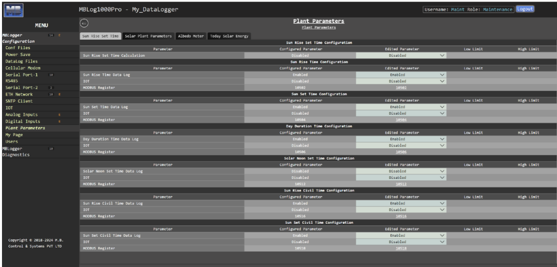
Figure-6.21: Configuration of Plant Parameters (special function).
