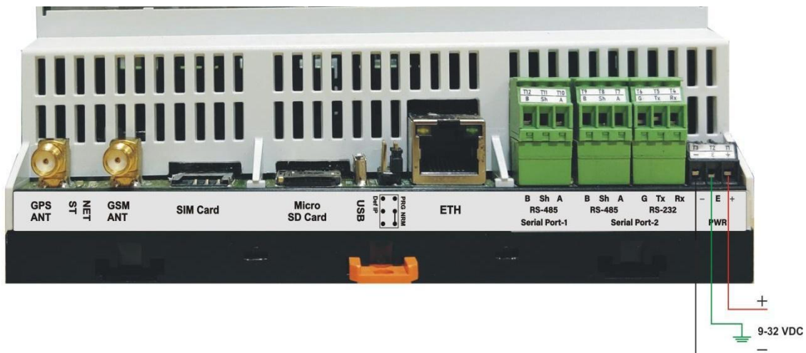
Figure-3.2: MBLLogger power supply connections.
