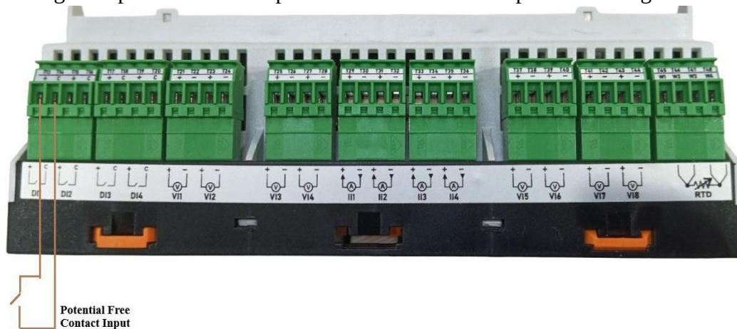
Figure-3.8.1: Digital input connections for potential free contacts.
