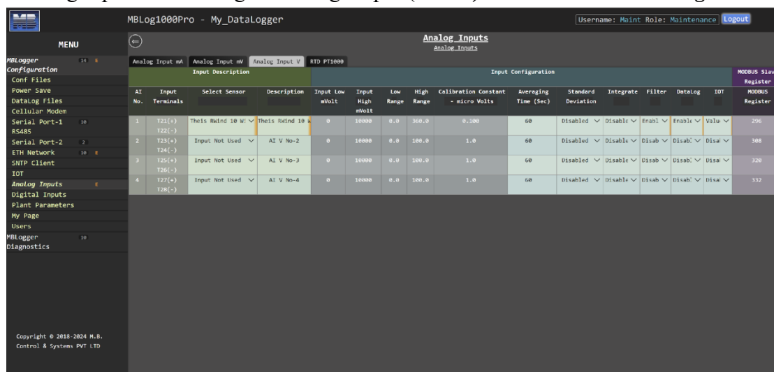
Figure-6.16.3: Configuration of Voltage input channels.
