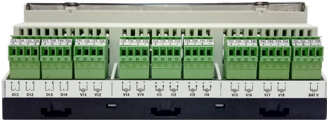
Figure-3.1.2: MBLLogger Signal input terminals (For Hardware version 2.11 and 3.11)
