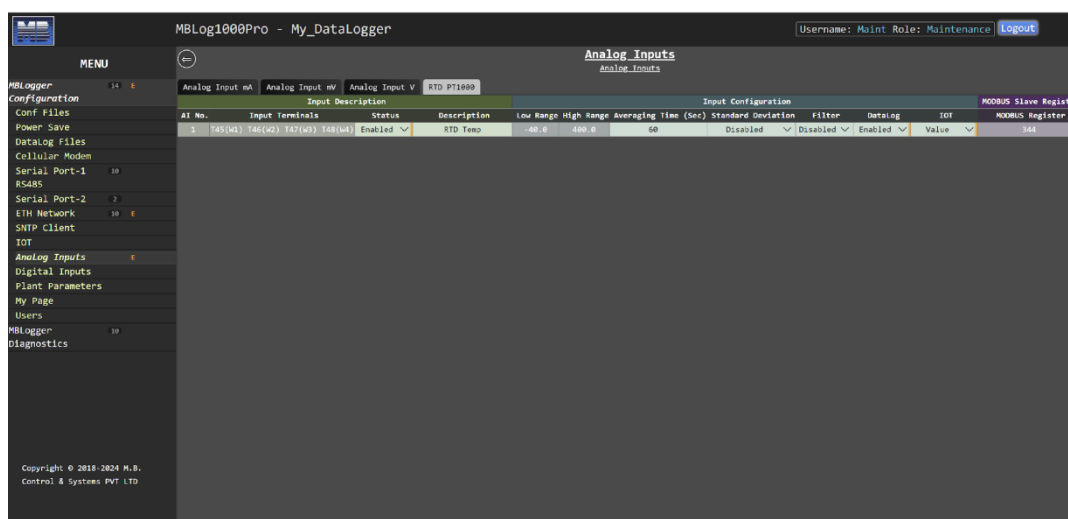
Figure-6.16.5: RTD input configuration.
