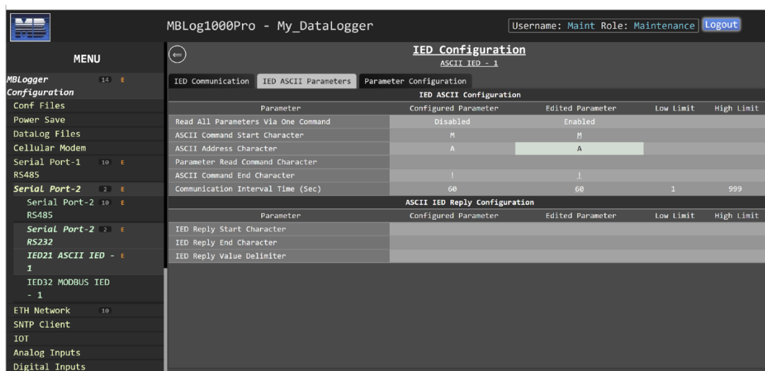
Figure-6.13.2: Configuration of IED ASCII communication parameters.
