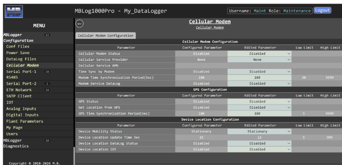
Figure-6.6: Configuration of internal cellular modem.
