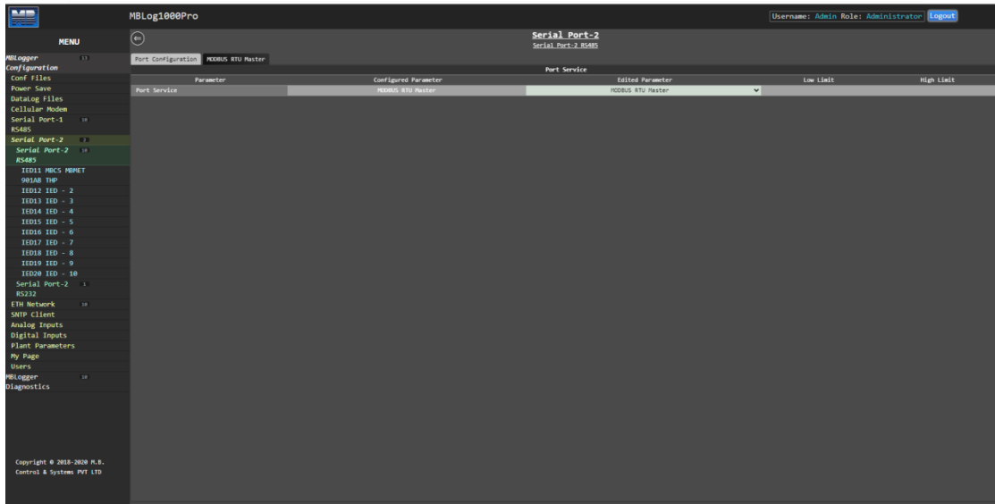
Figure-6.10.1: Configuration of serial port-2 RS485.
