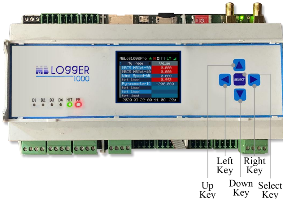
Figure-4.2: Datalogger keys
