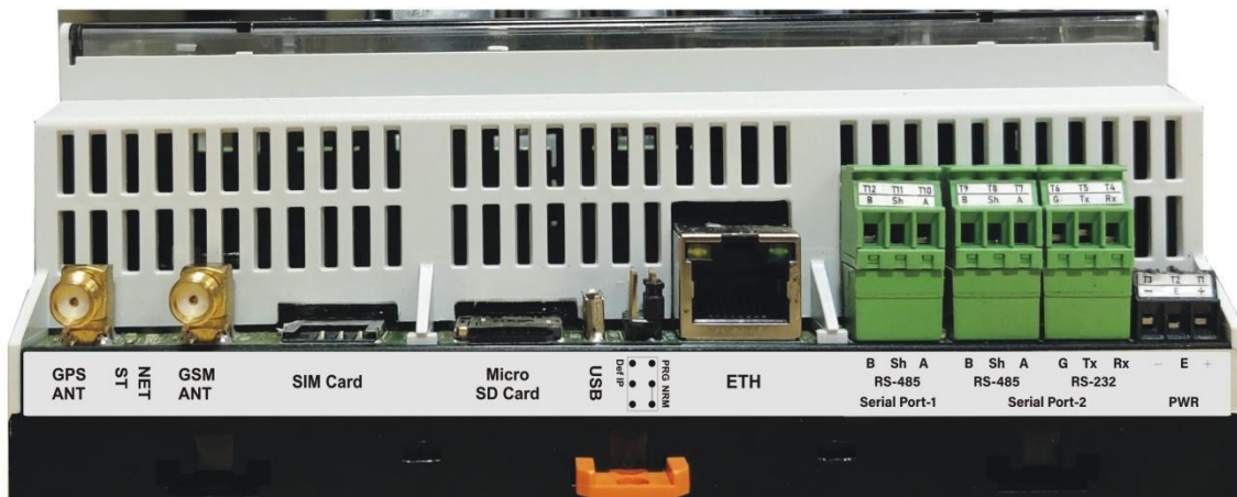
Figure-3.5.1: MBLLogger ETH Port.
