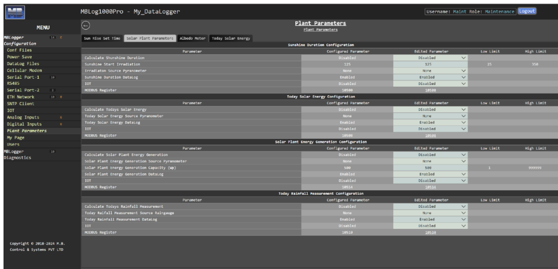
Figure-6.21.2: Configure Solar Plant Parameters.
