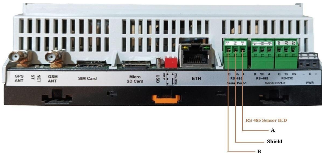
Figure-3.3: MBLLogger serial port-1 (RS485) connections.
