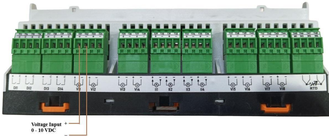
Figure-3.9: Measurement voltage (0-10VDC) input connections.
