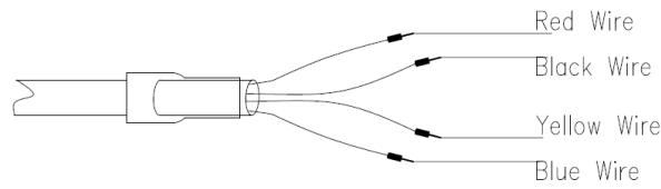
Fig: 4.1 – Wind Speed Sensor Wire
