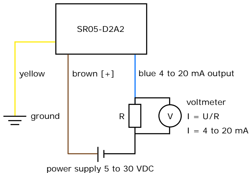
Figure 5.9.2 Electrical diagram of the connection of SR05-D2A2 to a typical voltmeter or datalogger with the capacity to measure voltage signals. Usually a 100 \Omega shunt resistor ( R ) is used to convert the current to a voltage. SR05-D2A2 operates on a supply voltage of 5 to 30 VDC.
