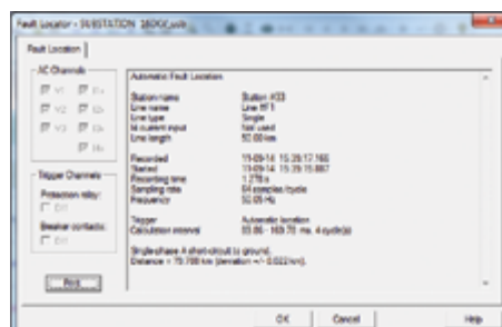
DISTANCE TO FAULT CALCULATION (PAS)
