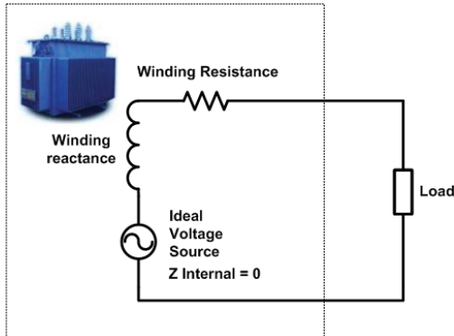
Figure 1: Simple Electrical Network
