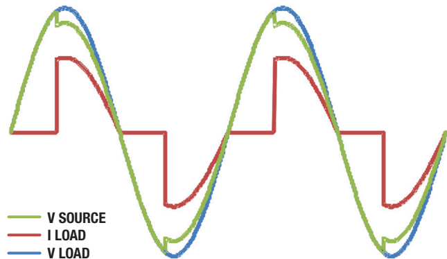
Figure 2: Distorted Waveform
