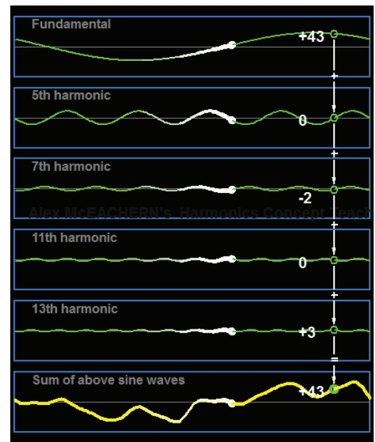
Figure 3: Adding Waveforms
