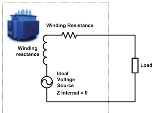
Figure 1: Simple Electrical Network
