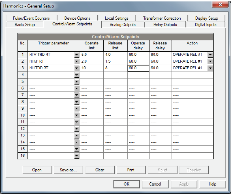
Figure 5: Harmonics Setup Example
