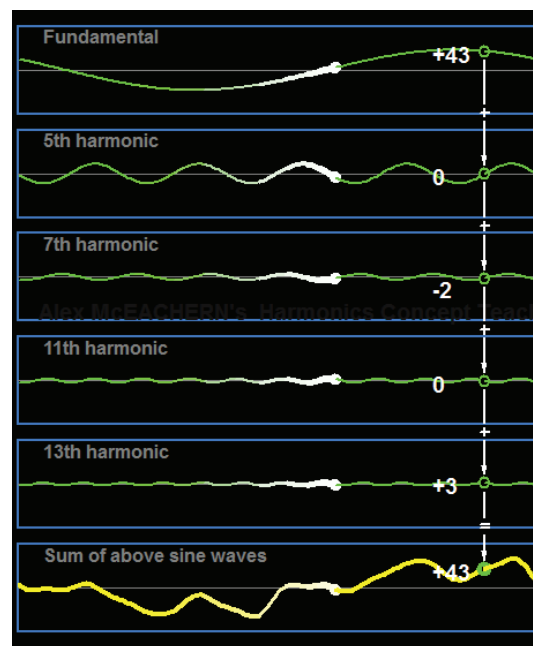
Figure 3: Adding Waveforms
