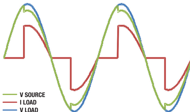
Figure 2: Distorted Waveform
