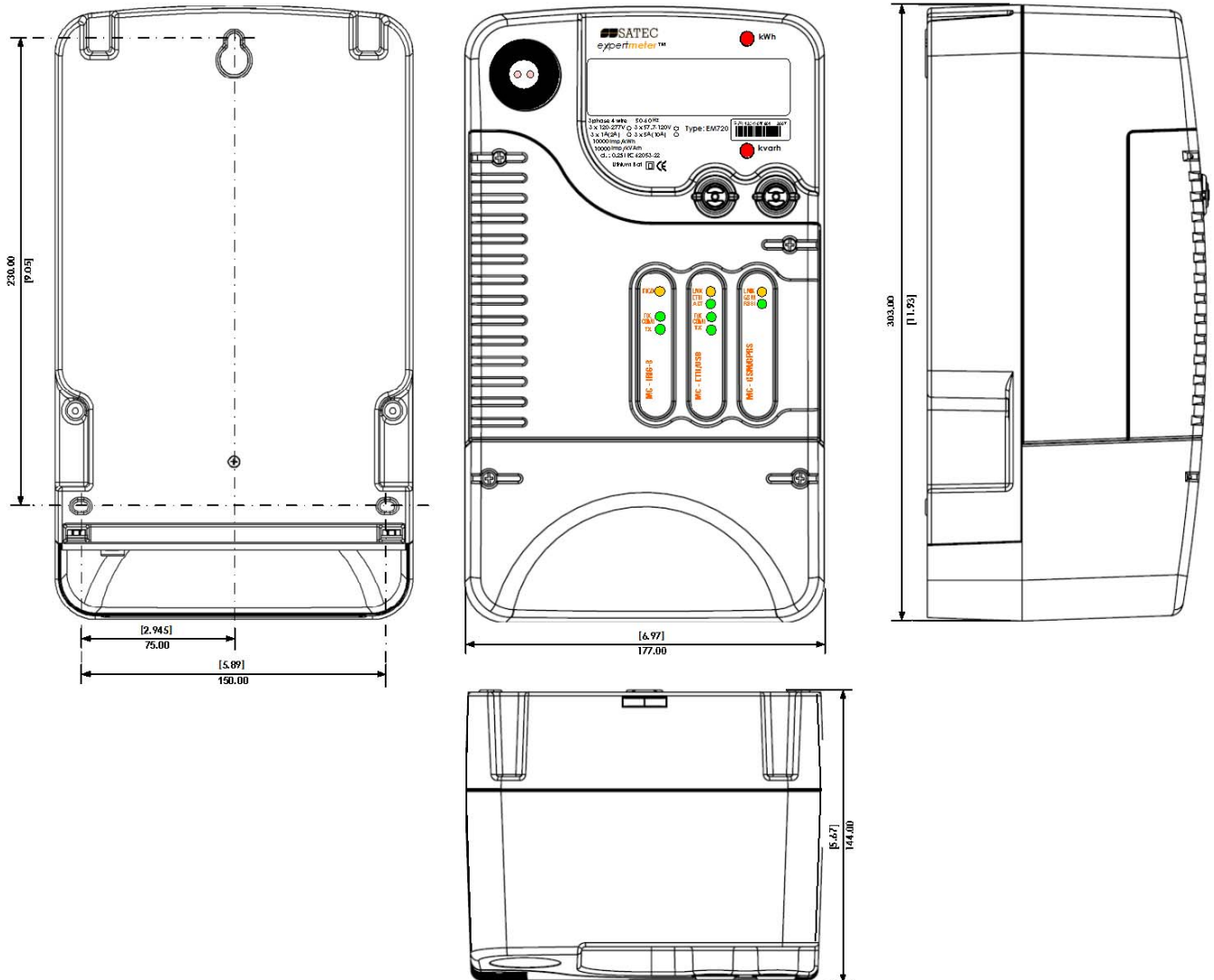
Figure 1: Dimensions
