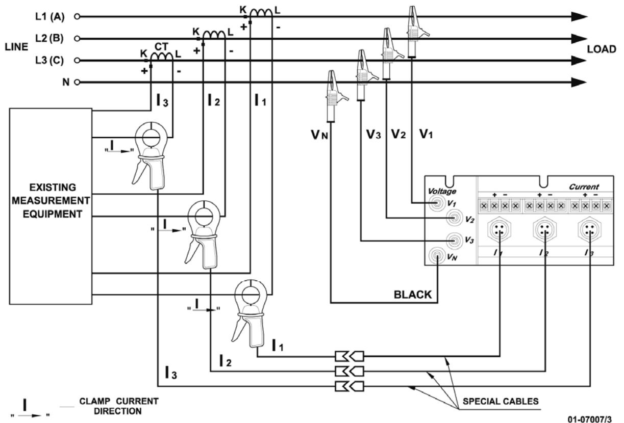
Figure 2-4 Four Wire WYE Direct Connection with special cables using 3 CTs (3-element) Wiring Mode = 4LL3 or 4Ln3
