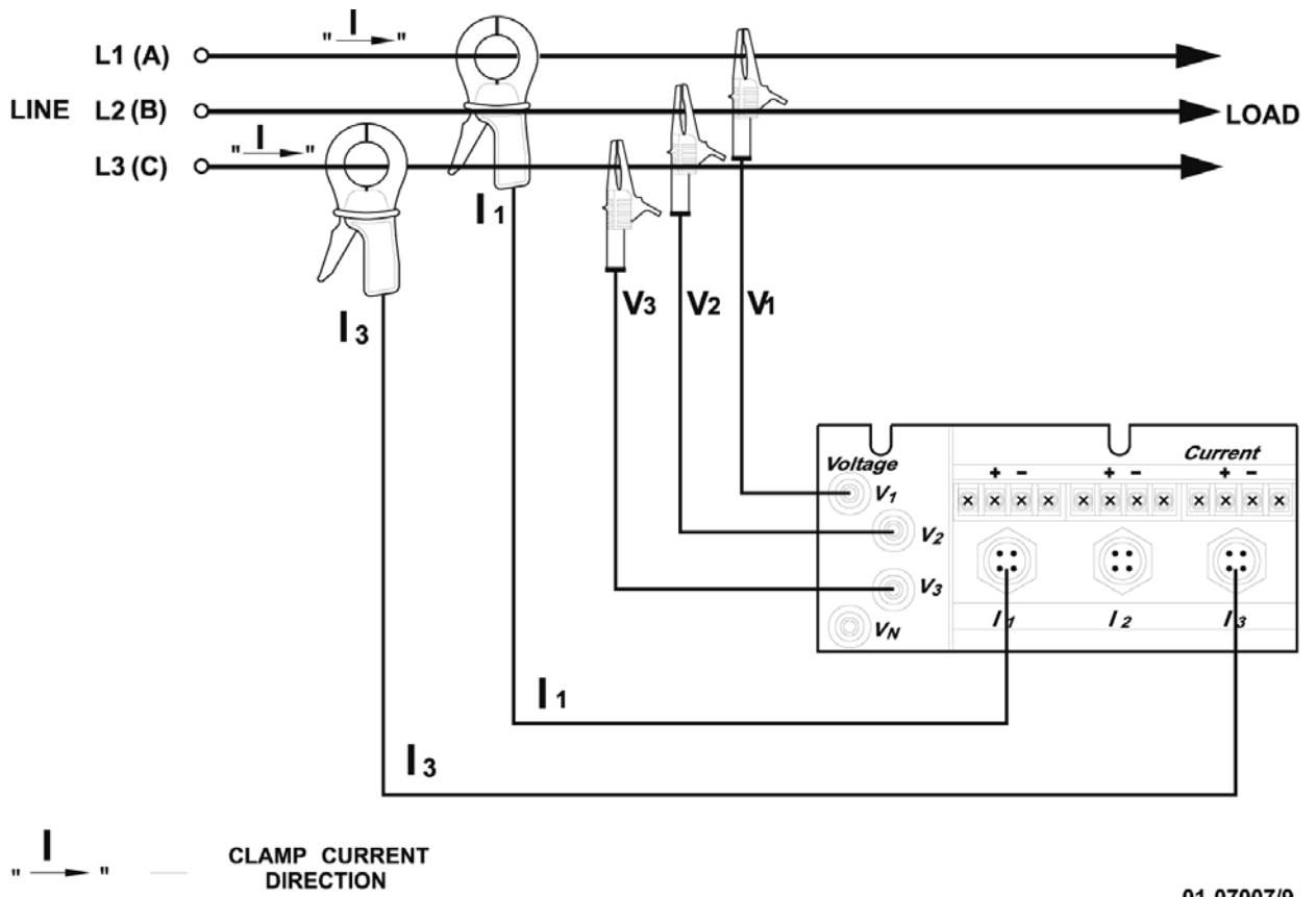
Figure 2-1 Three wire direct connection using 2 CTs (2-element), Wiring Mode=3dir2
