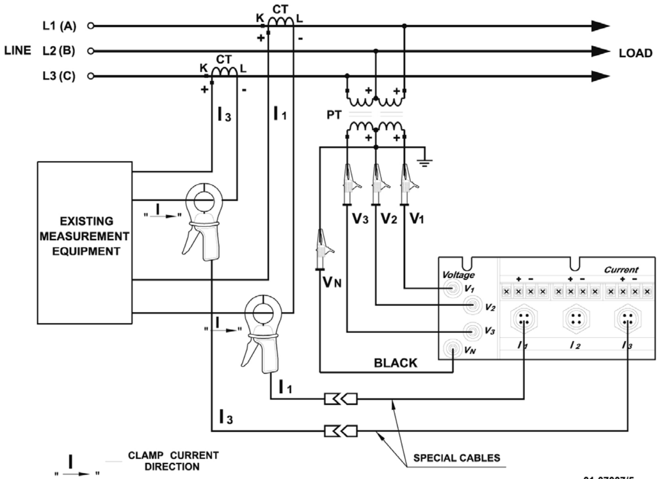
Figure 2-8 Three Wire Open Delta Connection with special cables using 2 PTs, 2 CTs (2-element) Wiring Mode = 3OP2
