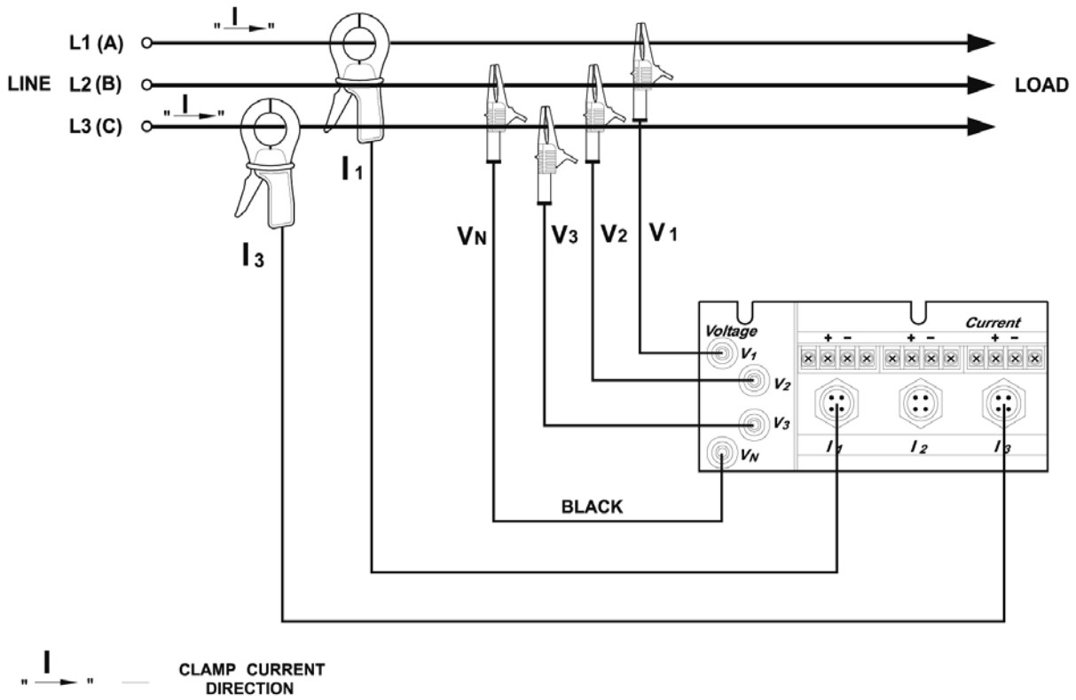
Figure 2-6 Three Wire Open Delta Connection using 2 PTs, 2 CTs (2-element) Wiring Mode = 3OP2
