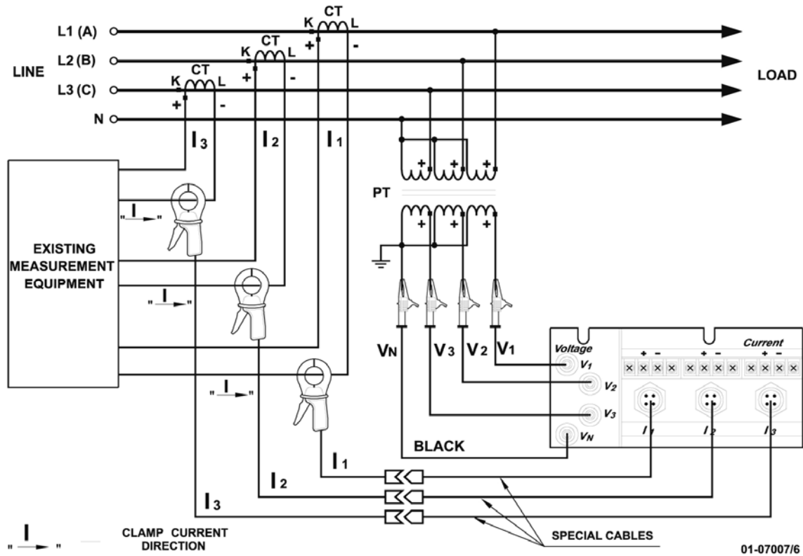
Figure 2-5 Four Wire WYE Connection with special cables using 3 PTs, 3 CTs (3-element) Wiring Mode = 4LL3 or 4Ln3
