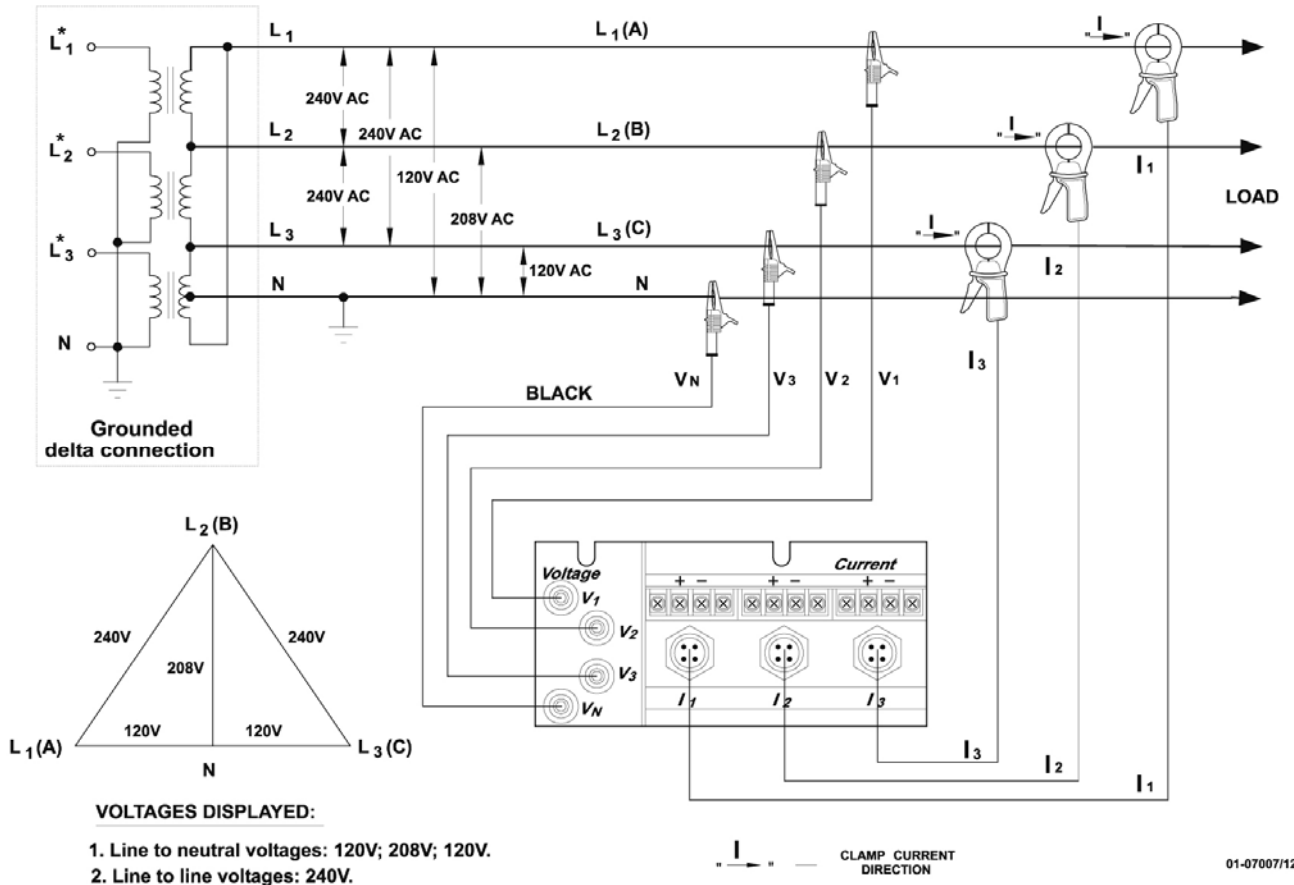
Figure 2-11 Four Wire Delta Direct Connection using 3 CTs (3 element) Wiring Mode = 4LL3 or 4Ln3
