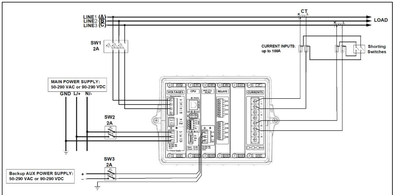
Figure 2-3 Three Wire Direct Connection Using 2 CTs (2-element)
