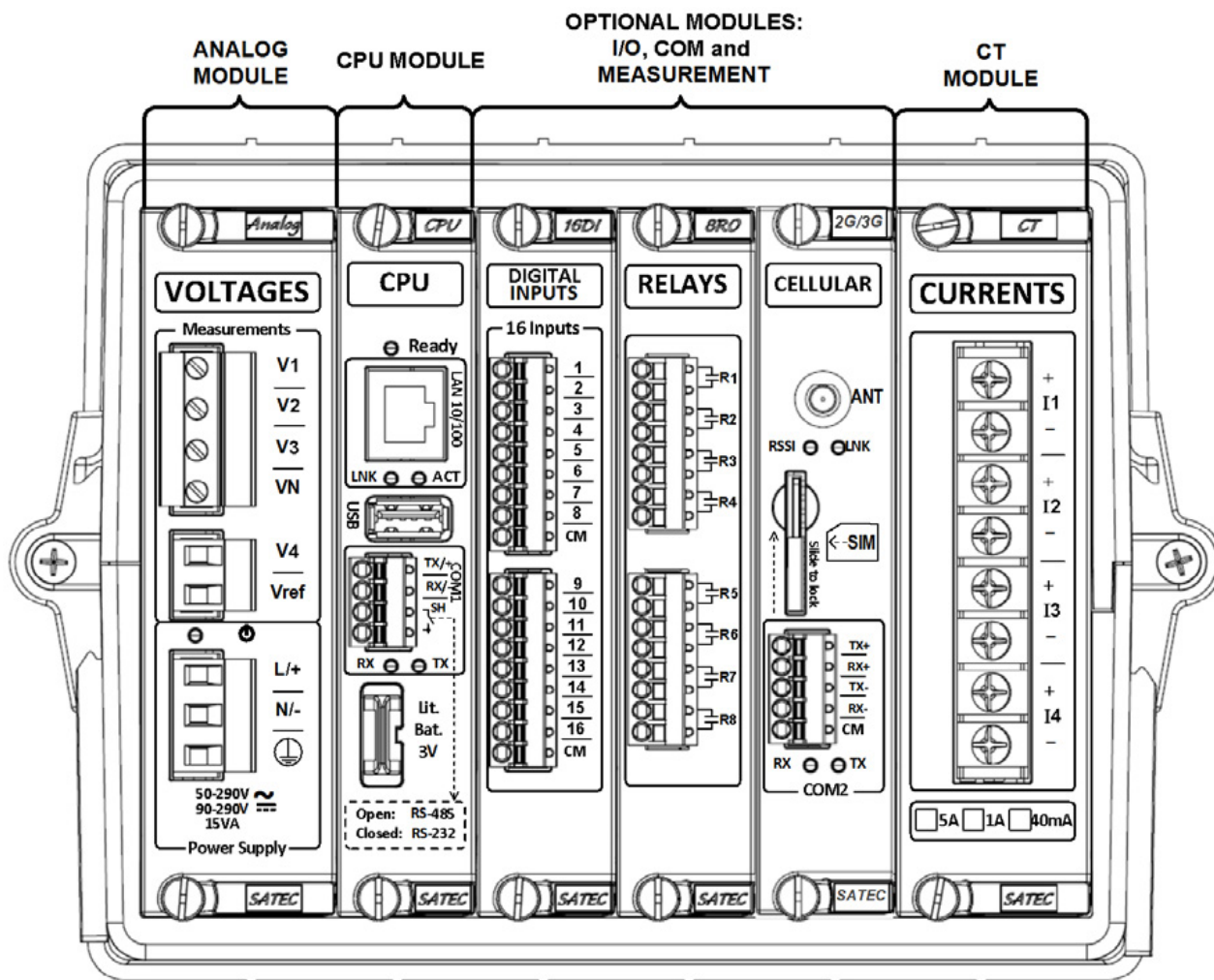
Figure 2-19 Location of Modules
