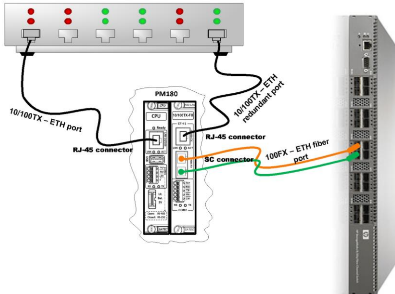
Figure 2-18 ETHERNET port Connection – RJ45 and SC
