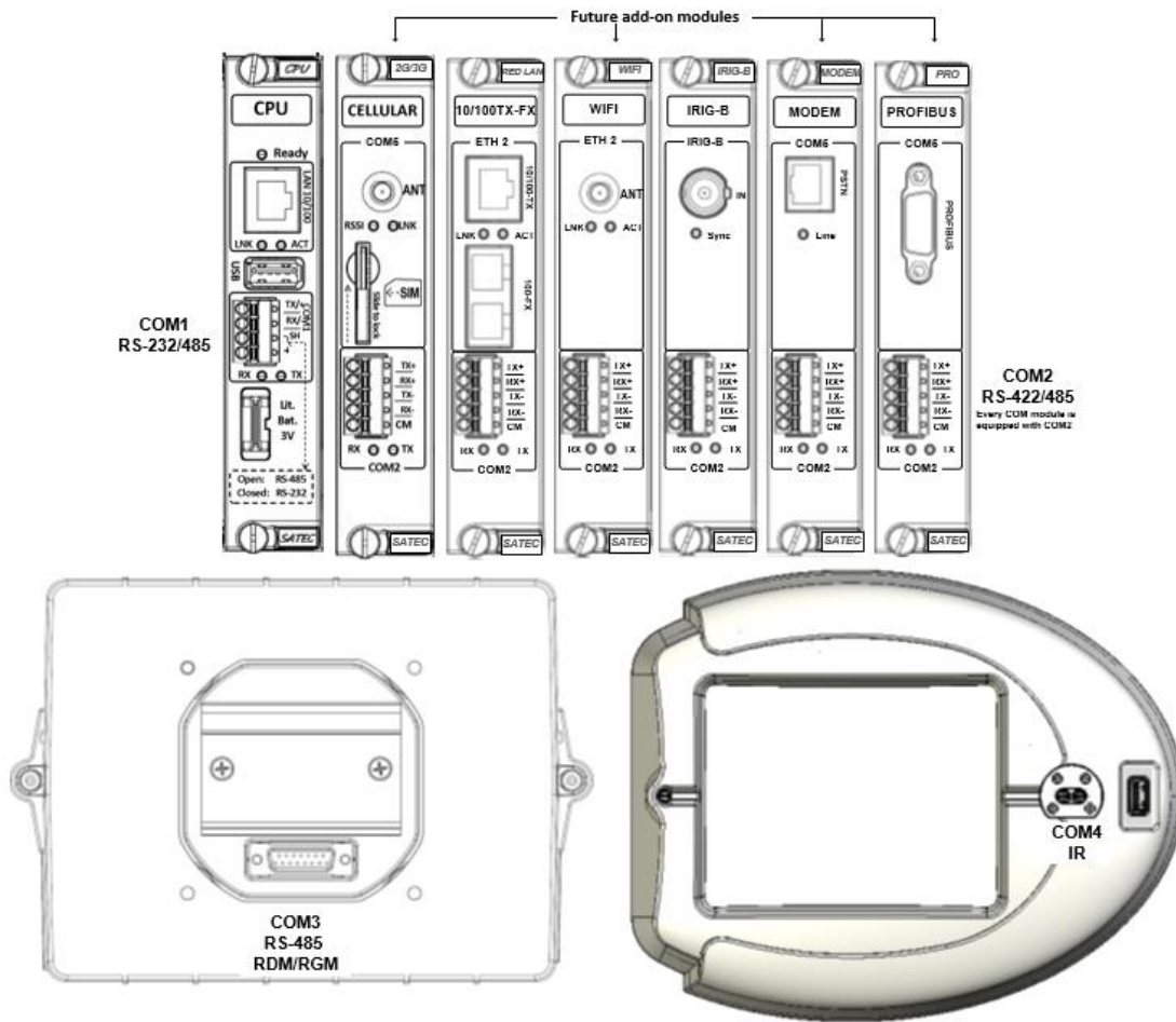
Figure 3-1 RS-232/RS-422/RS-485 ports location
