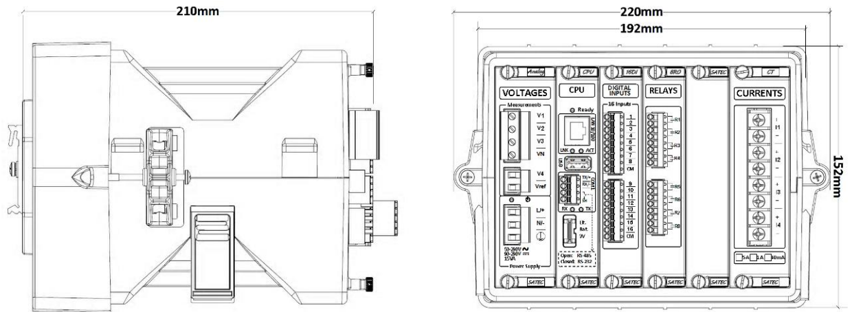
Figure 2-1a Dimensions
