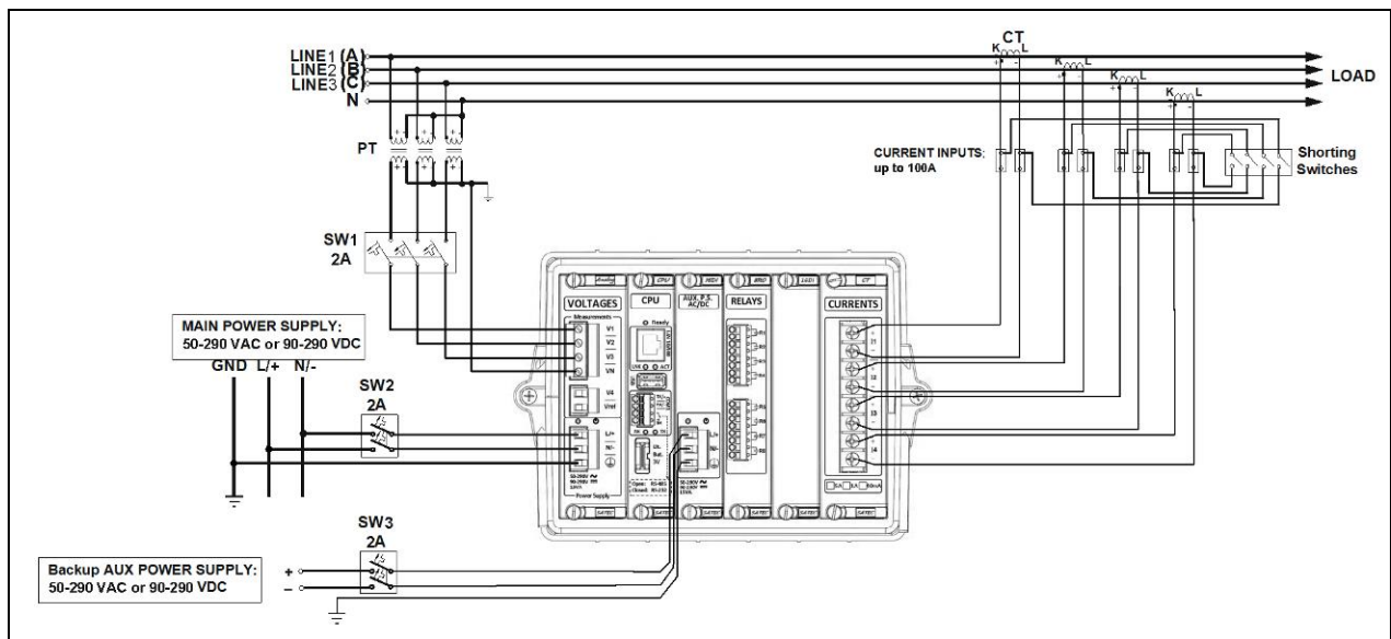
Figure 2-5a Four Wire WYE Connection Using 3 PTs, 4 CTs (3-element)
