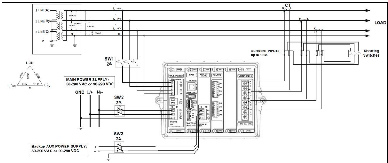
Figure 2-9 Four Wire Delta Direct Connection Using 3 CTs (3 element) Wiring Mode = 4LL3 or 4Ln3
