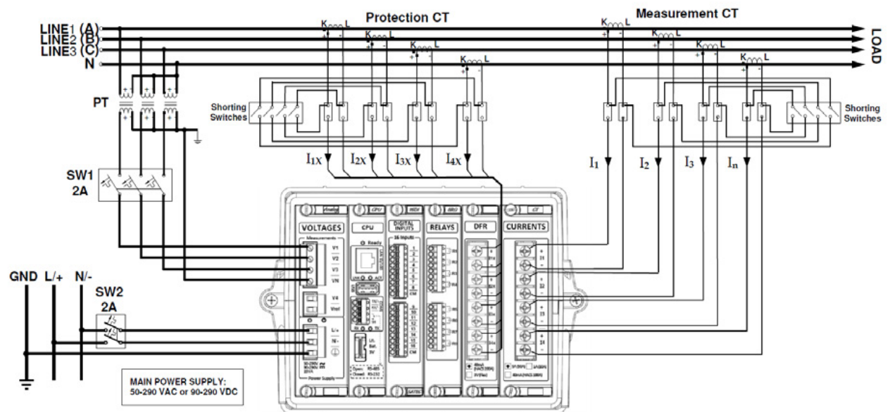
Figure 2-15 Digital Fault Recorder wiring installation
