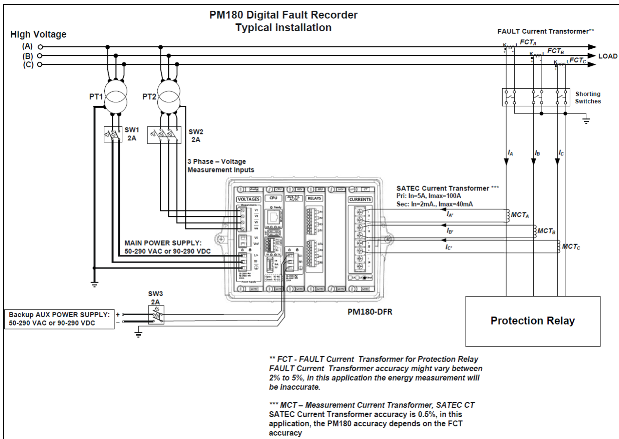
Figure 2-5b Four Wire WYE Connection Using 3 PTs, 3 CTs (3-element) for DFR Model (CS1S)
