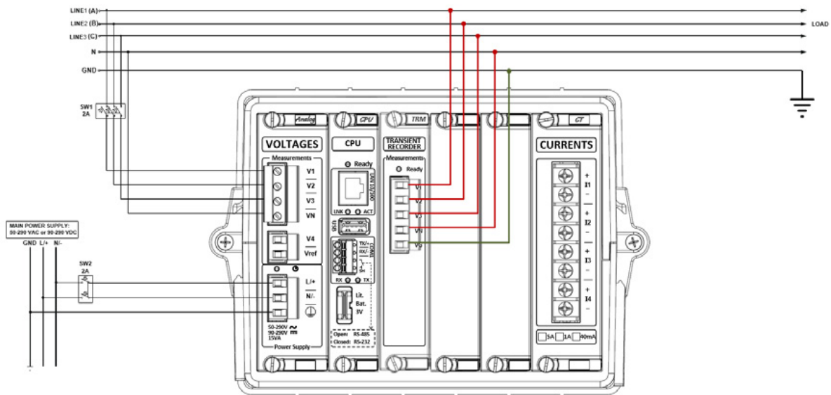
Figure 2-14 Transient Recorder wiring installation
