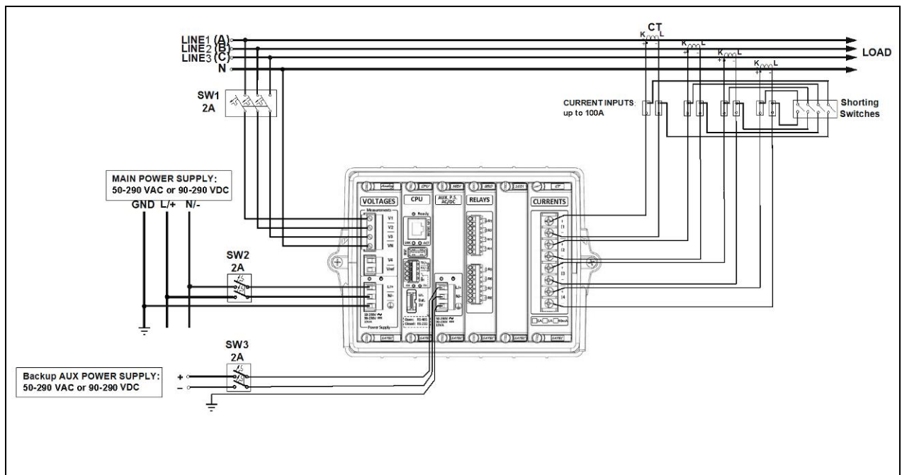
Figure 2-4 Four Wire WYE Direct Connection Using 4 CTs (3-element)
